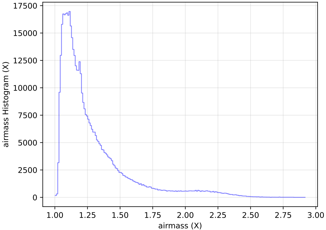
ddf_acor_sf15_Isf40_Isr20_v3.4_10yrs WFD r band: airmass Histogram
