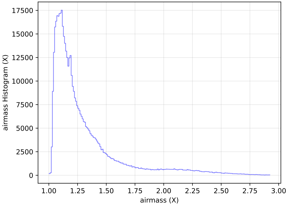
ddf_acor_sf15_lsf40_lsr20_v3.4_10yrs WFD i band: airmass Histogram
