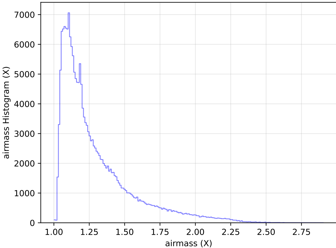
ddf_acor_sf15_lsf40_lsr20_v3.4_10yrs WFD g band: airmass Histogram
