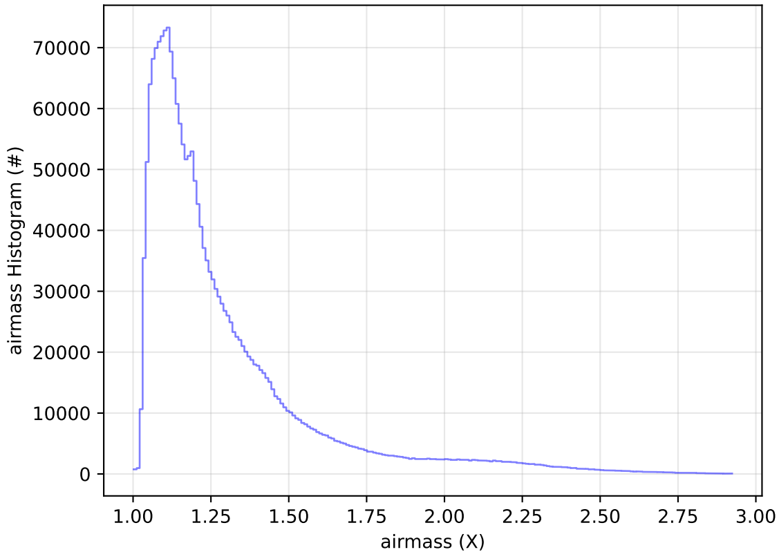
ddf_acor_sf15_lsf40_lsr20_v3.4_10yrs WFD all bands: airmass Histogram
