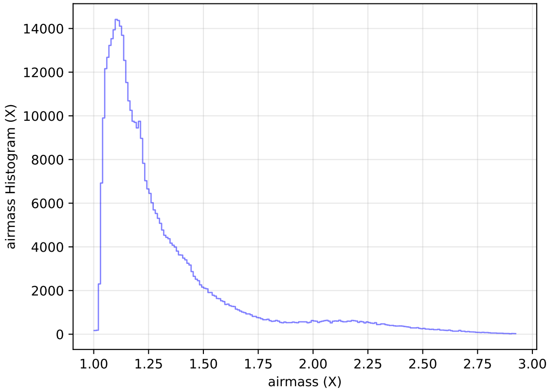
ddf_acor_sf15_lsf40_lsr20_v3.4_10yrs All sky z band: airmass Histogram
