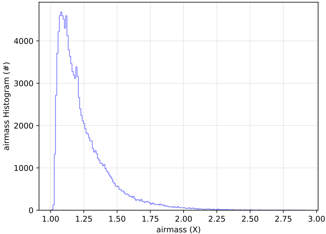
ddf_acor_sf15_lsf40_lsr20_v3.4_10yrs All sky u band: airmass Histogram
