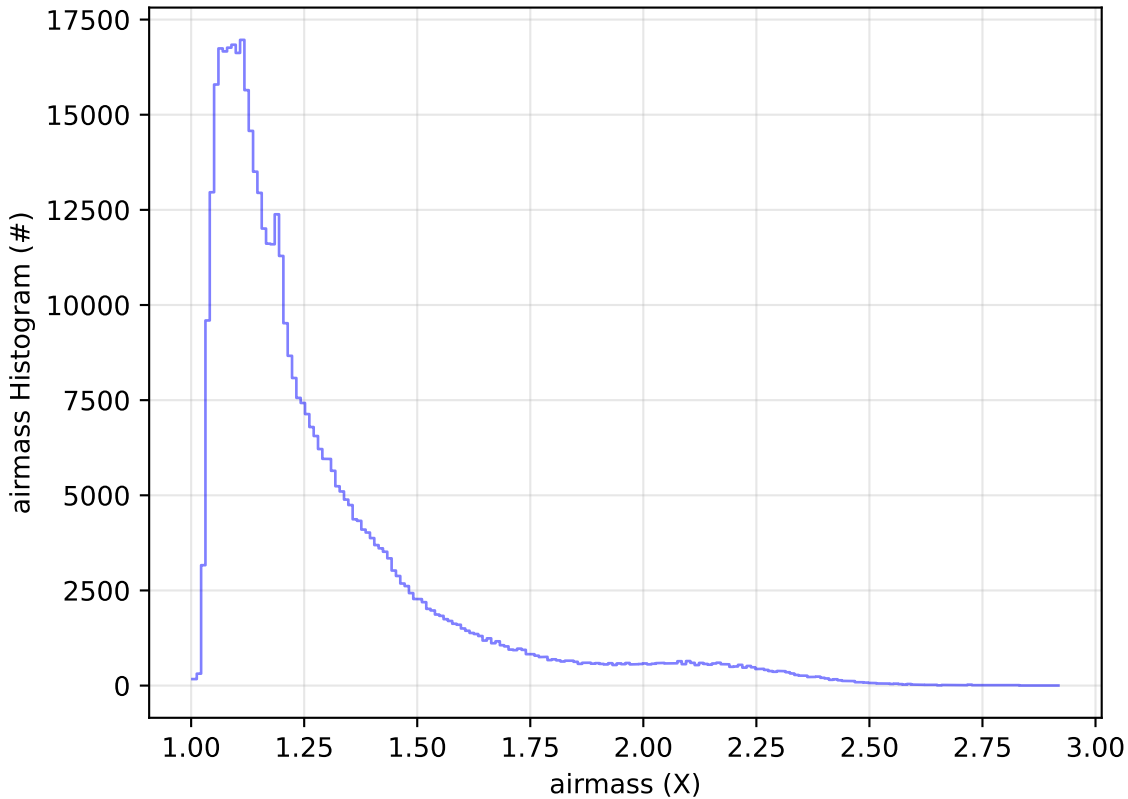
ddf_acor_sf15_lsf40_lsr20_v3.4_10yrs All sky r band: airmass Histogram
