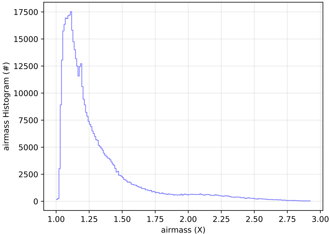
ddf_acor_sf15_lsf40_lsr20_v3.4_10yrs All sky i band: airmass Histogram
