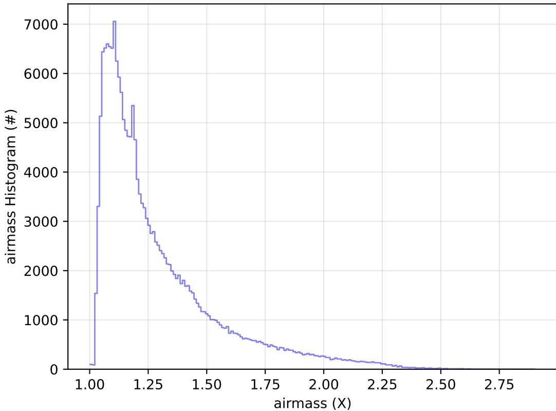
ddf_acor_sf15_lsf40_lsr20_v3.4_10yrs All sky g band: airmass Histogram
