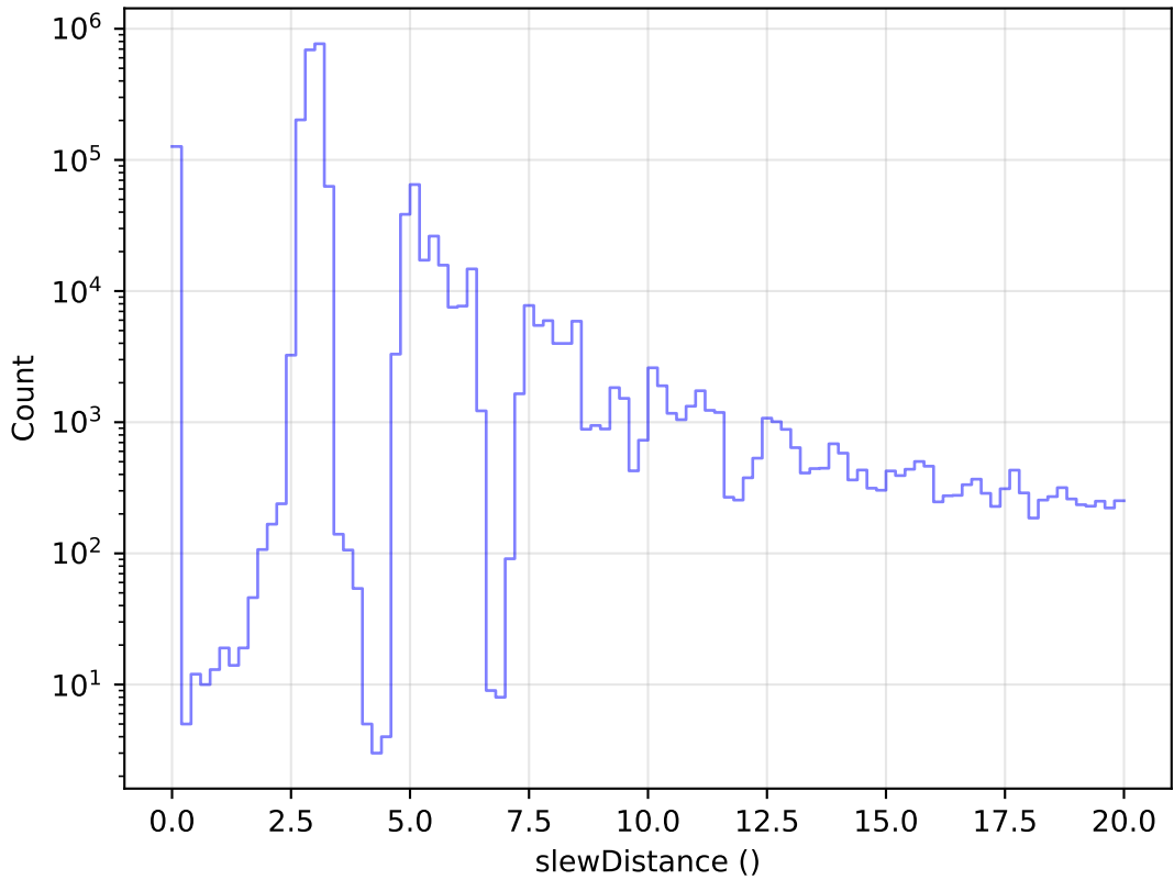
ddf_acor_sf15_lsf40_lsr20_v3.4_10yrs All visits: Zoom Slew Distance Histogram
