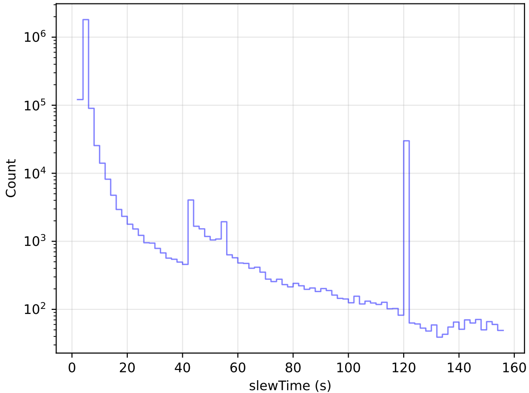
ddf_acor_sf15_lsf40_lsr20_v3.4_10yrs All visits: Slew Time Histogram
