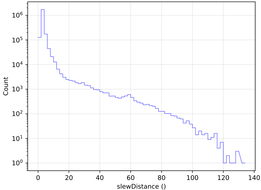
ddf_acor_sf15_lsf40_lsr20_v3.4_10yrs All visits: Slew Distance Histogram
