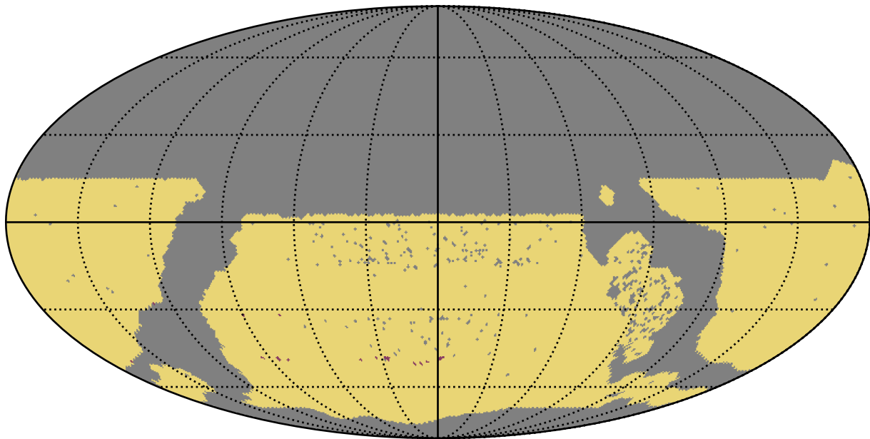
ddf_acor_sf15_lsf40_lsr20_v3.4_10yrs WFD: RapidRevisits
