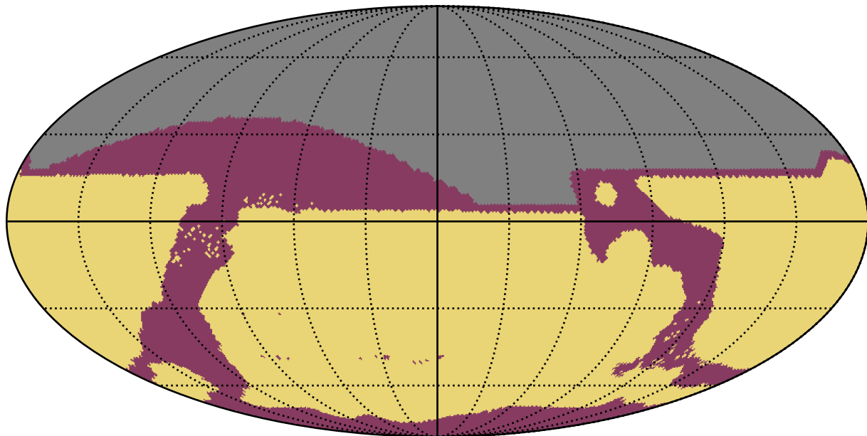
ddf_acor_sf15_lsf40_lsr20_v3.4_10yrs All sky: RapidRevisits
