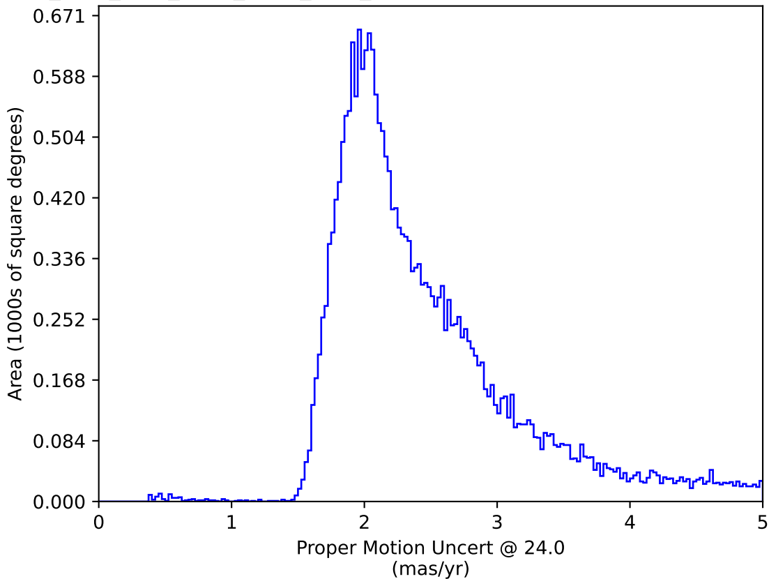
ddf_acor_sf15_lsf40_lsr20_v3.4_10yrs All sky: Proper Motion Uncert @ 24.0
