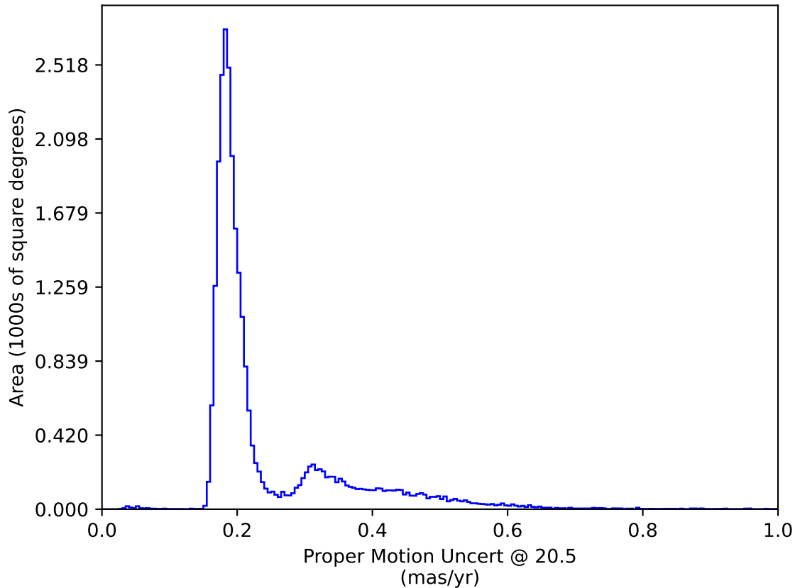
ddf_acor_sf15_lsf40_lsr20_v3.4_10yrs All sky: Proper Motion Uncert @ 20.5
