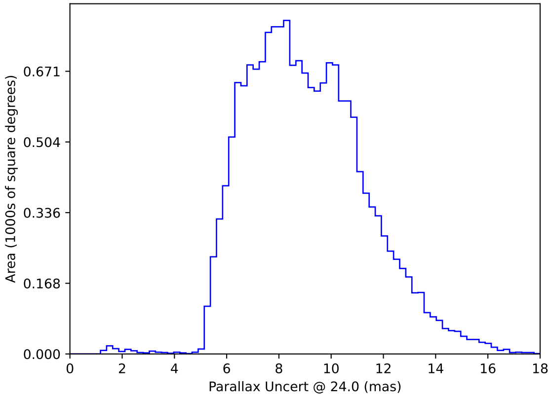
ddf_acor_sf15_lsf40_lsr20_v3.4_10yrs WFD: Parallax Uncert @ 24.0
