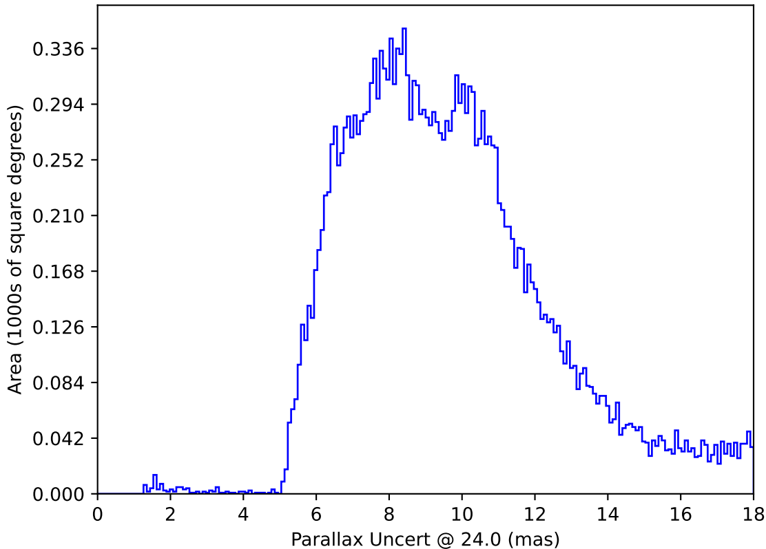
ddf_acor_sf15_lsf40_lsr20_v3.4_10yrs All sky: Parallax Uncert @ 24.0
