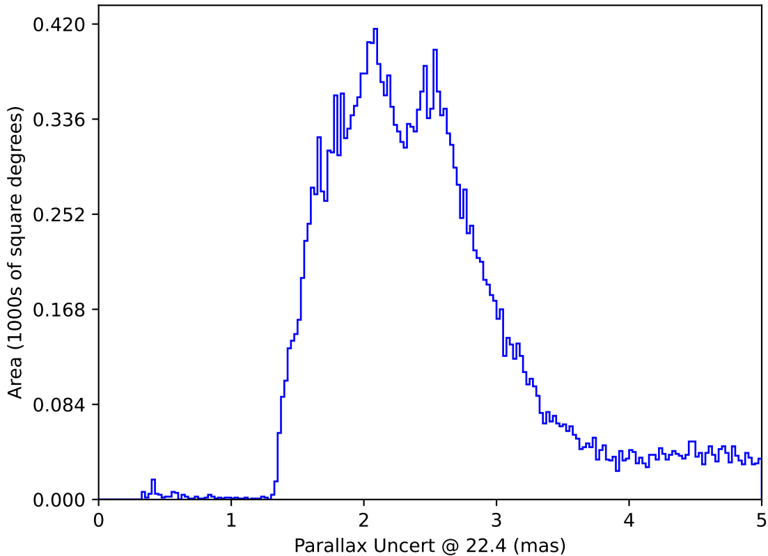
ddf_acor_sf15_lsf40_lsr20_v3.4_10yrs All sky: Parallax Uncert @ 22.4
