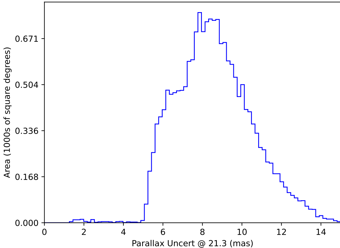
ddf_acor_sf15_lsf40_lsr20_v3.4_10yrs WFD y band only: Parallax Uncert @ 21.3
