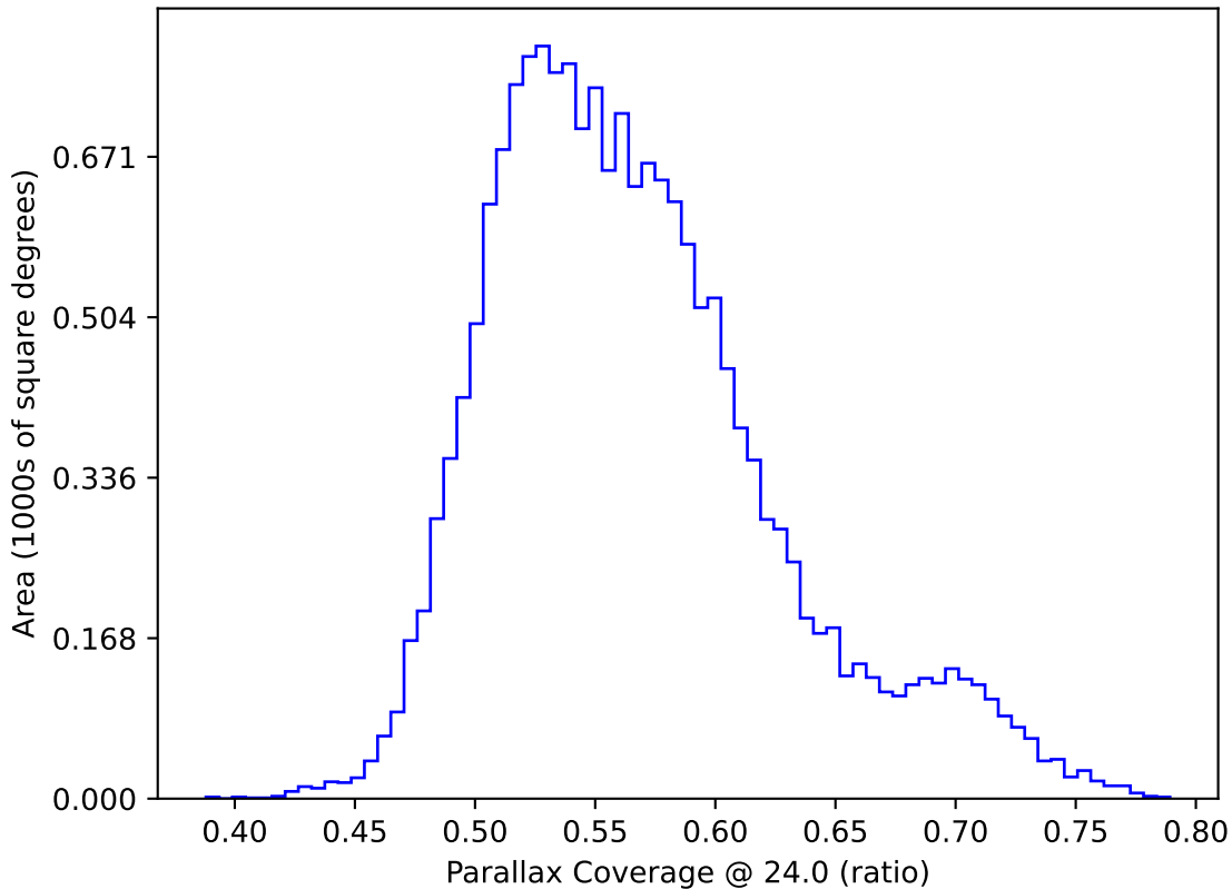
ddf_acor_sf15_lsf40_lsr20_v3.4_10yrs WFD: Parallax Coverage @ 24.0
