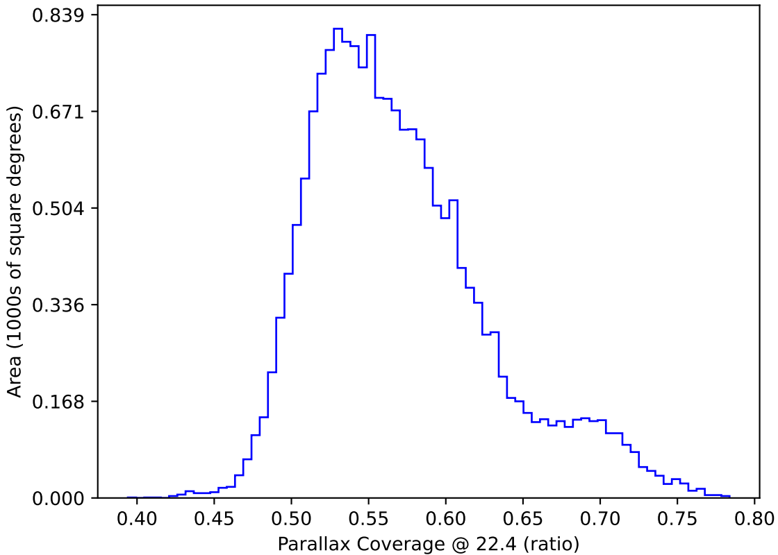
ddf_acor_sf15_lsf40_lsr20_v3.4_10yrs WFD: Parallax Coverage @ 22.4
