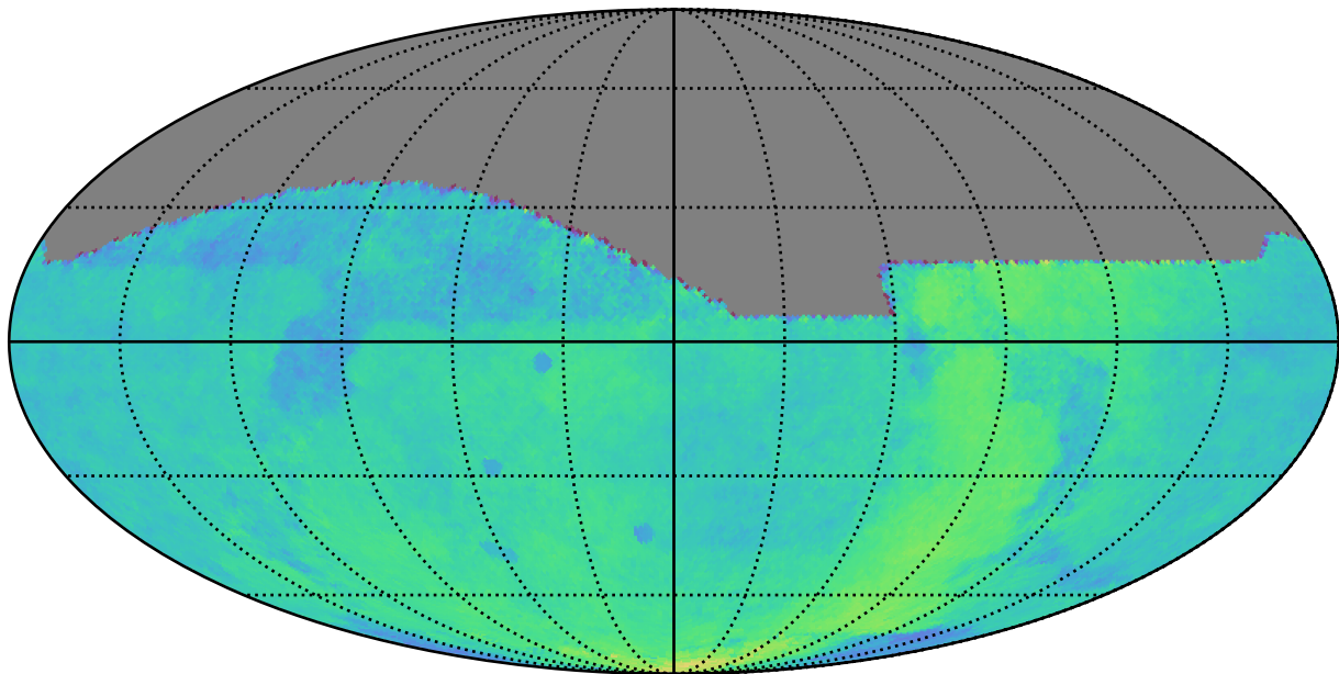
ddf_acor_sf15_lsf40_lsr20_v3.4_10yrs All sky: Parallax Coverage @ 22.4
