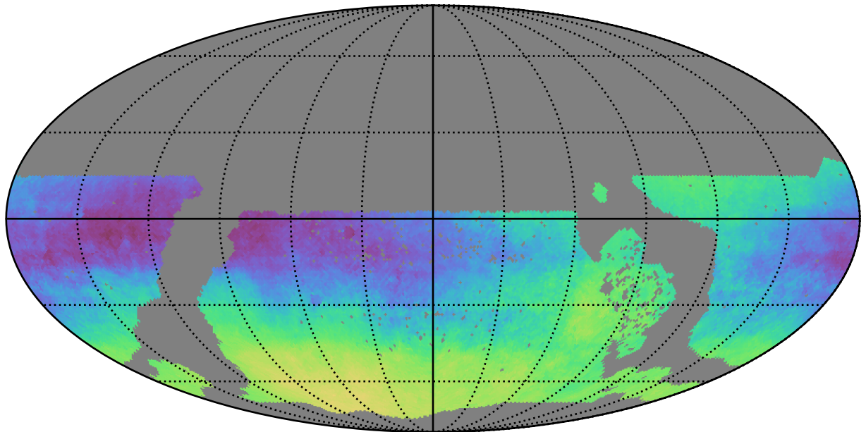
ddf_acor_sf15_lsf40_lsr20_v3.4_10yrs WFD: Parallax-DCR degeneracy @ 24.0
