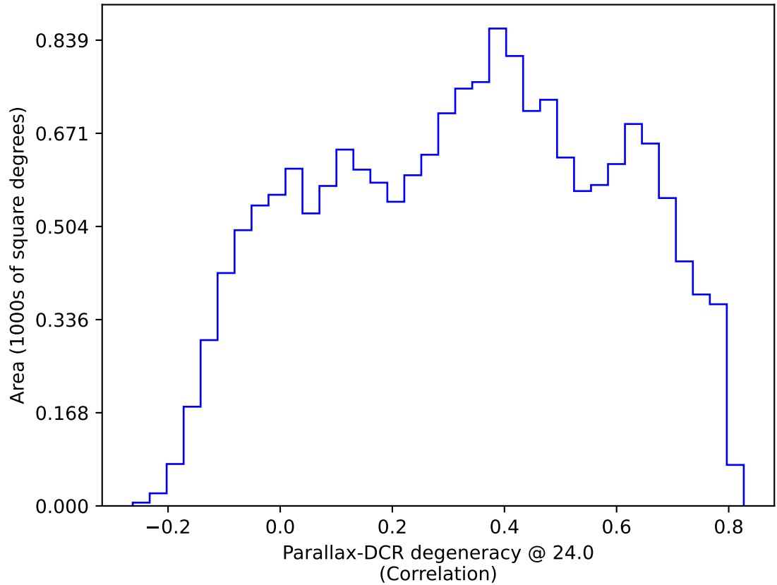
ddf_acor_sf15_lsf40_lsr20_v3.4_10yrs WFD: Parallax-DCR degeneracy @ 24.0
