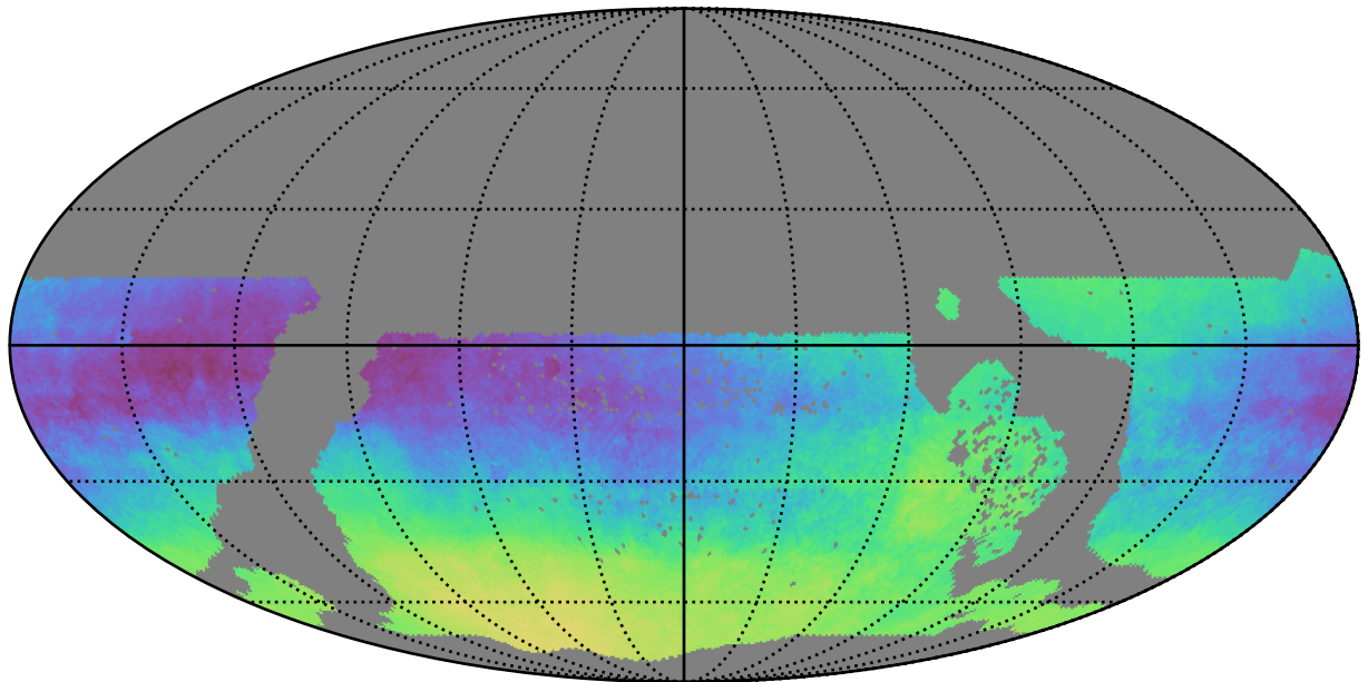
ddf_acor_sf15_lsf40_lsr20_v3.4_10yrs WFD: Parallax-DCR degeneracy @ 22.4
