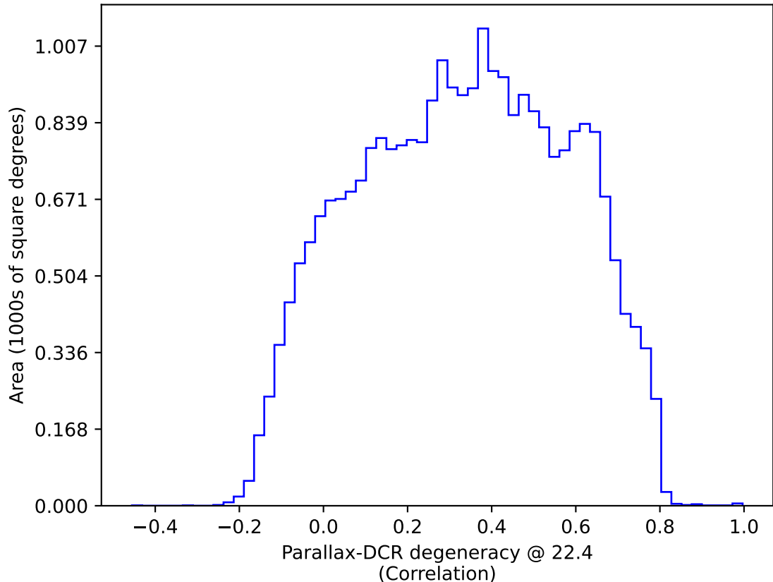
ddf_acor_sf15_lsf40_lsr20_v3.4_10yrs All sky: Parallax-DCR degeneracy @ 22.4
