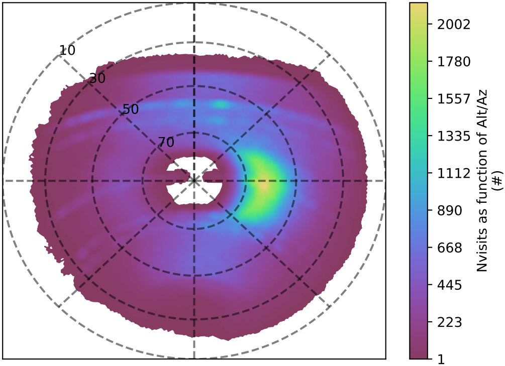
ddf_acor_sf15_lsf40_lsr20_v3.4_10yrs y band: Nvisits as function of Alt/Az
