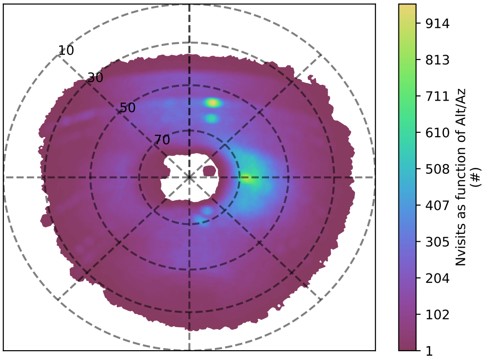
ddf_acor_sf15_lsf40_lsr20_v3.4_10yrs u band: Nvisits as function of Alt/Az
