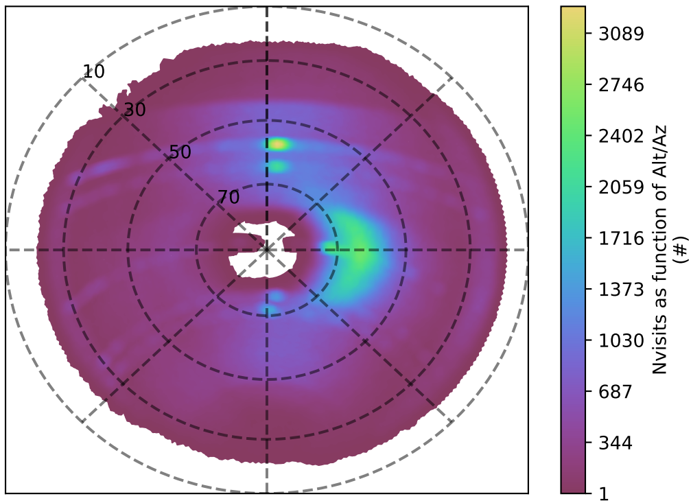
ddf_acor_sf15_lsf40_lsr20_v3.4_10yrs i band: Nvisits as function of Alt/Az
