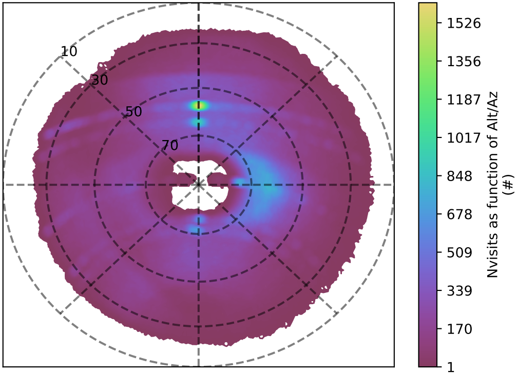
ddf_acor_sf15_lsf40_lsr20_v3.4_10yrs g band: Nvisits as function of Alt/Az
