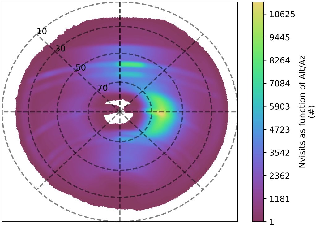
ddf_acor_sf15_ls40_lsr20_v3.4_10yrs all bands: Nvisits as function of Alt/Az
