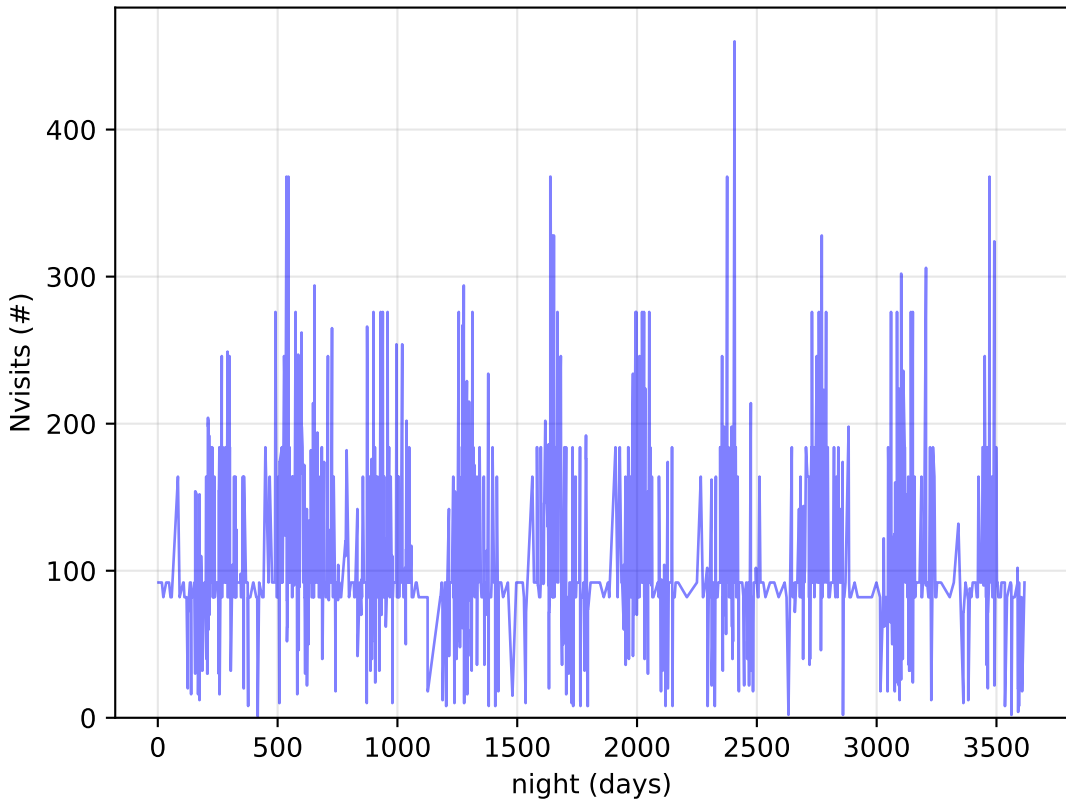
ddf_acor_sf15_lsf40_lsr20_v3.4_10yrs DDF: Nvisits
