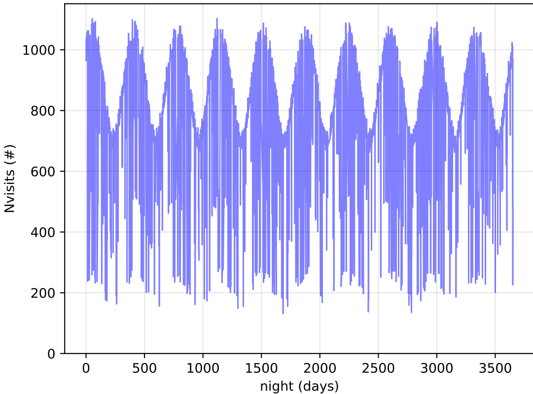
ddf_acor_sf15_lsf40_lsr20_v3.4_10yrs All visits: Nvisits
