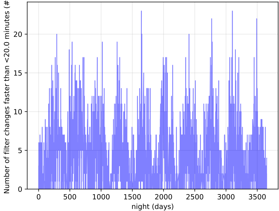
ddf_acor_sf15_Isf40_Isr20_v3.4_10yrs Per Night: Number of filter changes faster than <20.0 minutes
