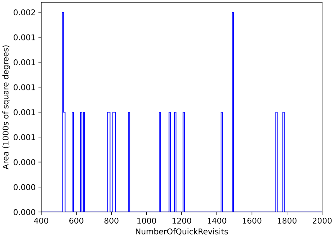
ddf_acor_sf15_lsf40_lsr20_v3.4_10yrs WFD: NumberOfQuickRevisits
