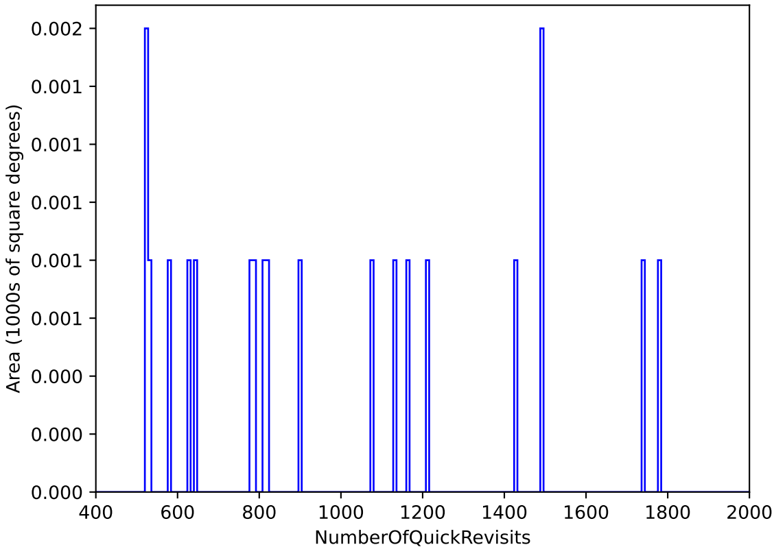
ddf_acor_sf15_lsf40_lsr20_v3.4_10yrs All sky: NumberOfQuickRevisits
