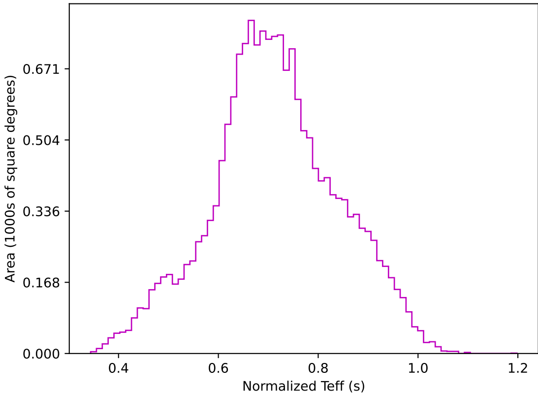
ddf_acor_sf15_lsf40_lsr20_v3.4_10yrs WFD z band: Normalized Teff
