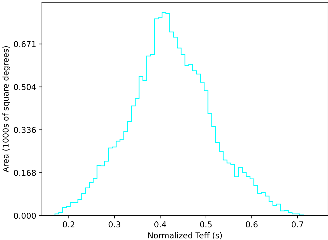
ddf_acor_sf15_lsf40_lsr20_v3.4_10yrs WFD u band: Normalized Teff
