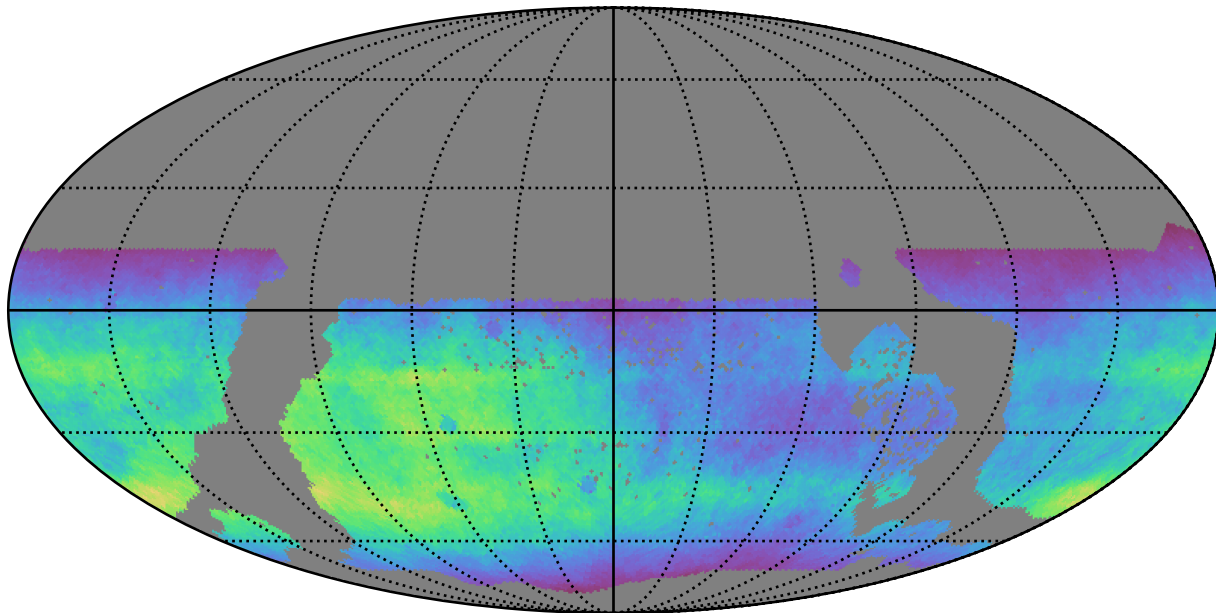
ddf_acor_sf15_lsf40_lsr20_v3.4_10yrs WFD r band: Normalized Teff
