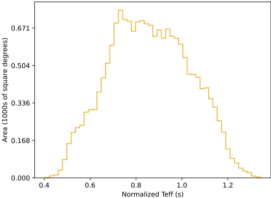
ddf_acor_sf15_lsf40_lsr20_v3.4_10yrs WFD r band: Normalized Teff
