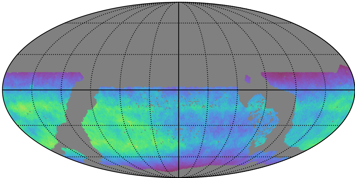
ddf_acor_sf15_lsf40_lsr20_v3.4_10yrs WFD i band: Normalized Teff
