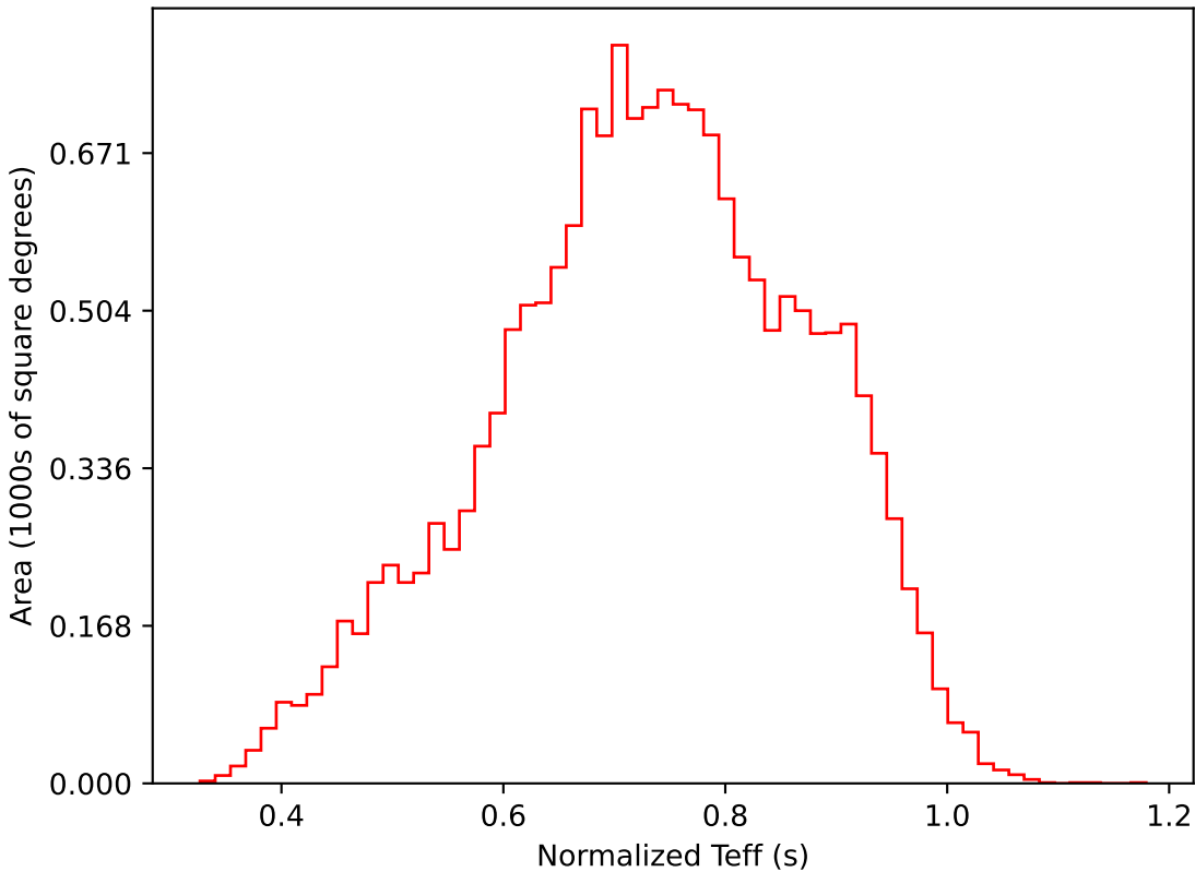
ddf_acor_sf15_lsf40_lsr20_v3.4_10yrs WFD i band: Normalized Teff
