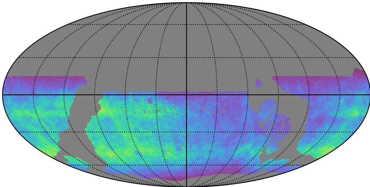
ddf_acor_sf15_lsf40_lsr20_v3.4_10yrs WFD g band: Normalized Teff
