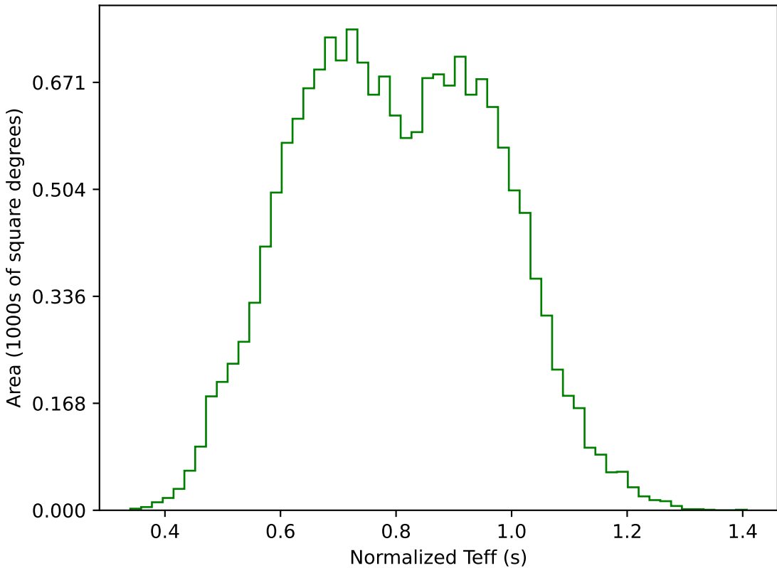
ddf_acor_sf15_lsf40_lsr20_v3.4_10yrs WFD g band: Normalized Teff
