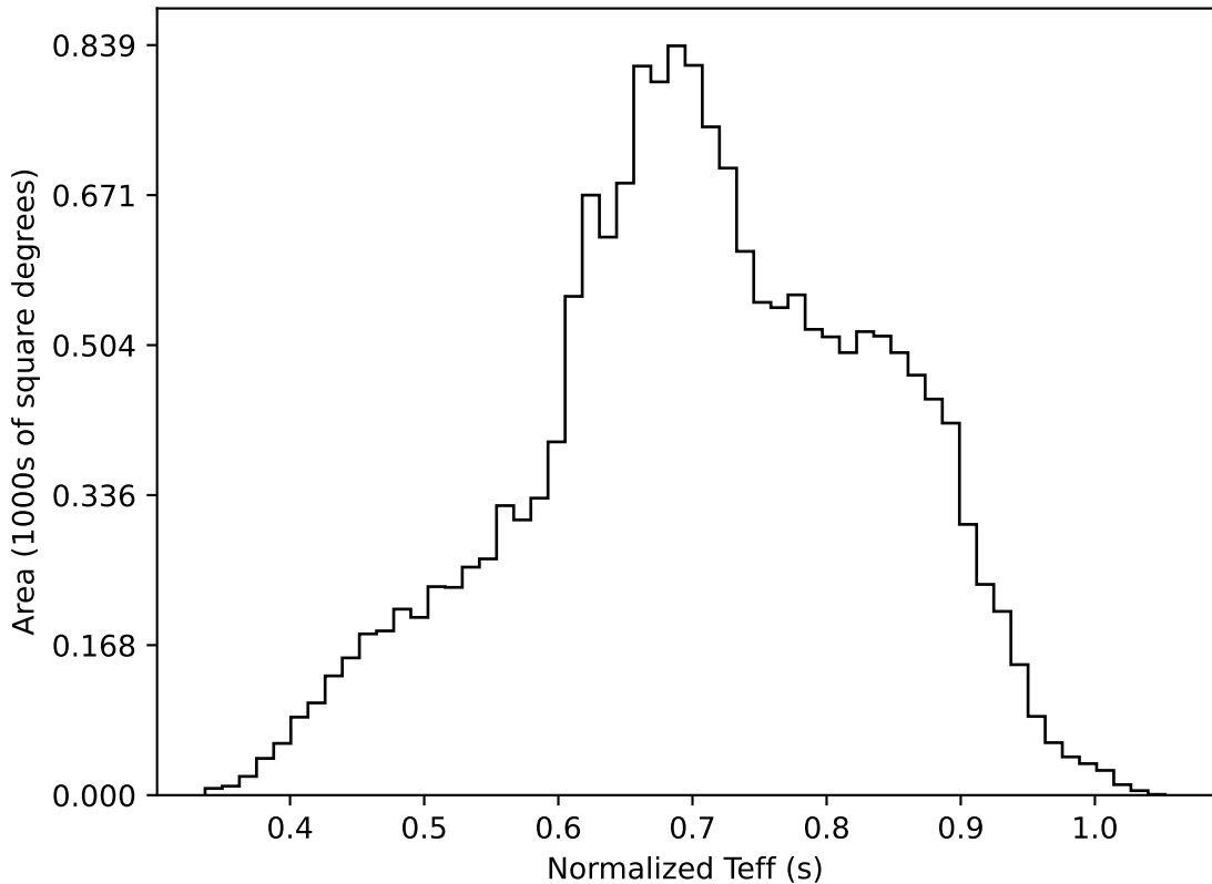
ddf_acor_sf15_lsf40_lsr20_v3.4_10yrs WFD all bands: Normalized Teff
