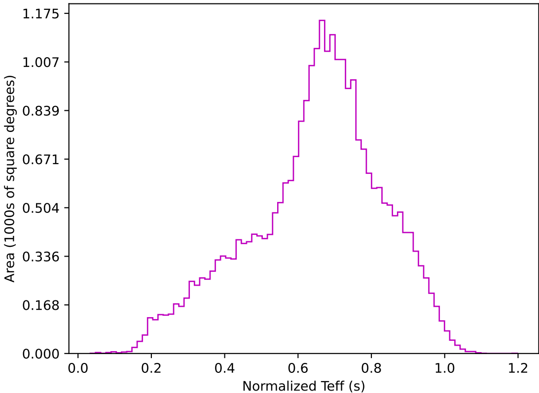
ddf_acor_sf15_lsf40_lsr20_v3.4_10yrs All sky z band: Normalized Teff
