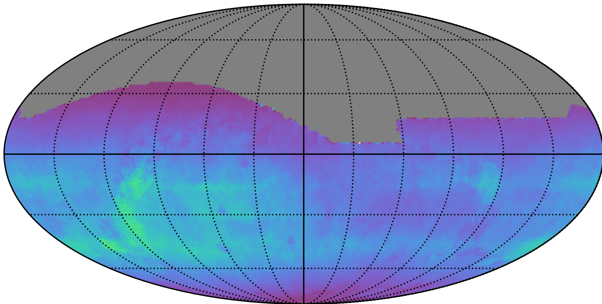
ddf_acor_sf15_lsf40_lsr20_v3.4_10yrs All sky r band: Normalized Teff
