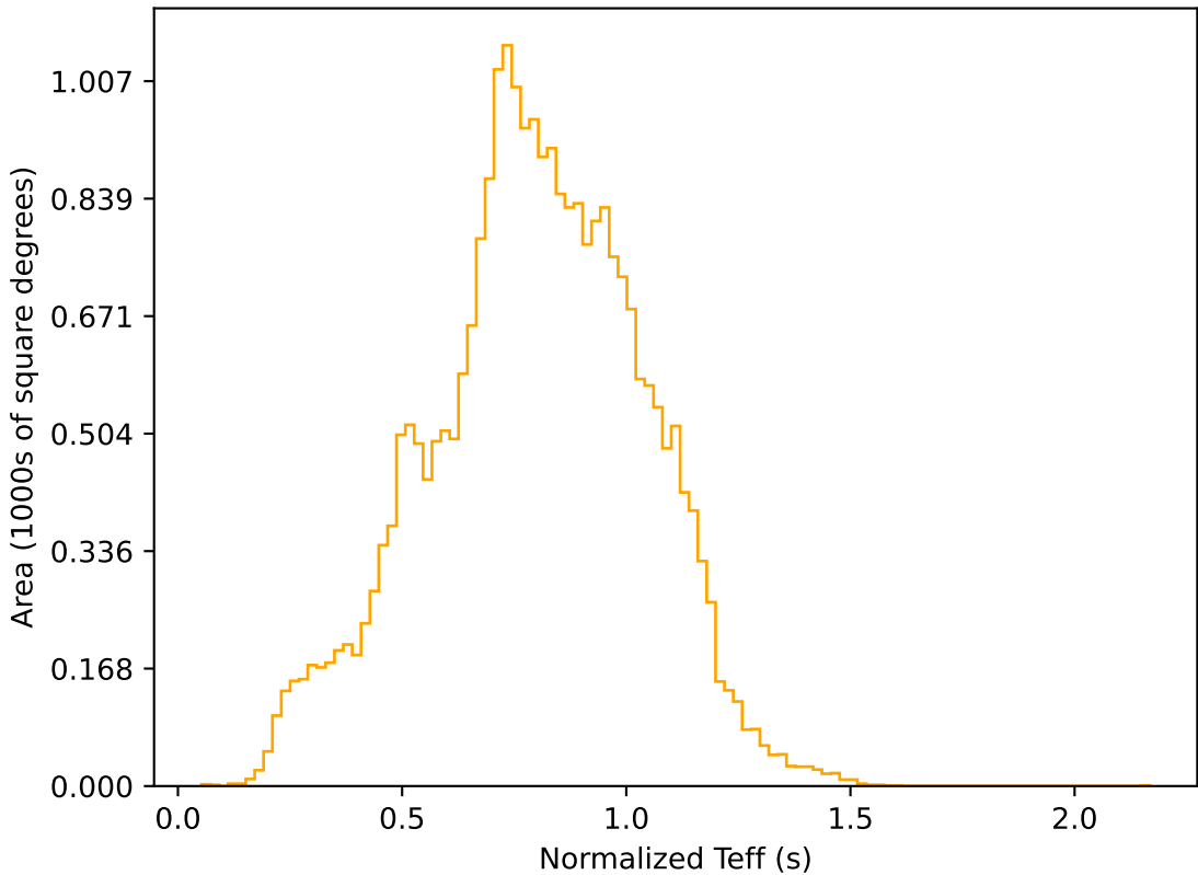
ddf_acor_sf15_lsf40_lsr20_v3.4_10yrs All sky r band: Normalized Teff
