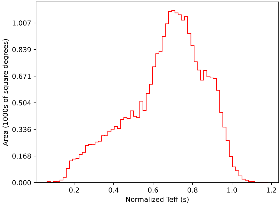
ddf_acor_sf15_lsf40_lsr20_v3.4_10yrs All sky i band: Normalized Teff
